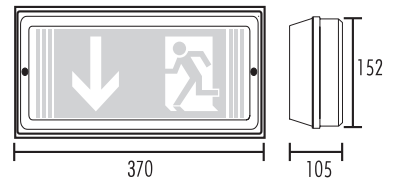
208W, Wandmontage
